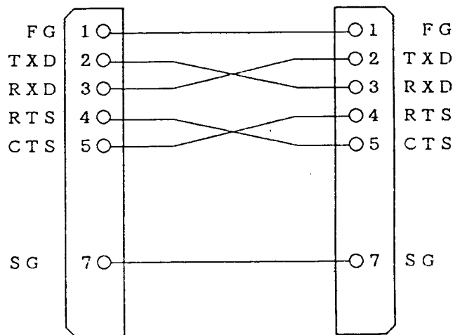
Fig. 10-2 Wiring diagram of the RS-232C interface cable
