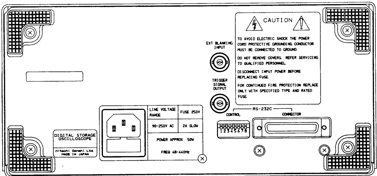
Fig. 4-1 (c) Rear View (VC-6025/6045)
