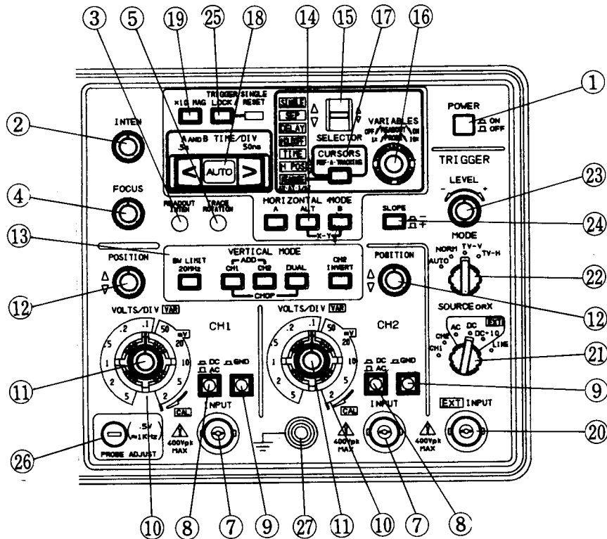
Fig. 5-1 Front Panel A section
