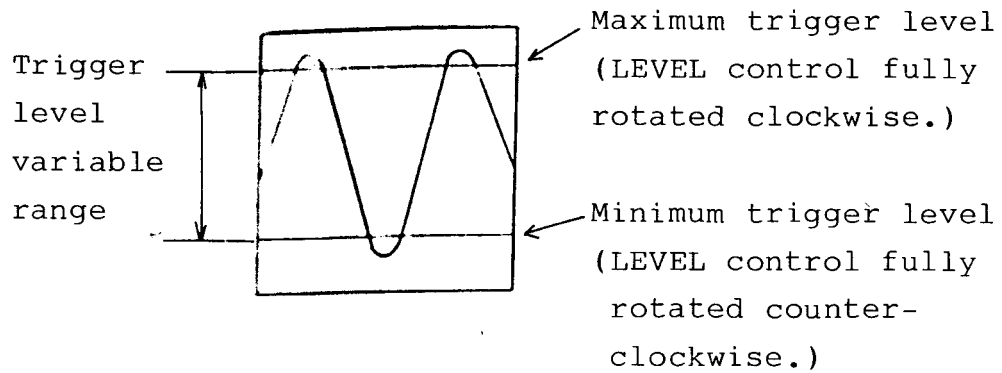
(a) Input signal of large amplitude
