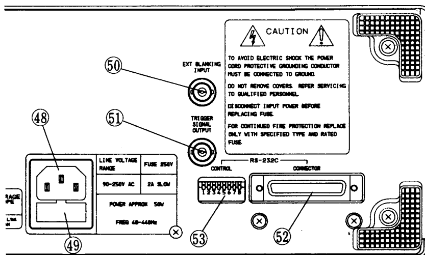
Fig. 5-3 Rear panel
